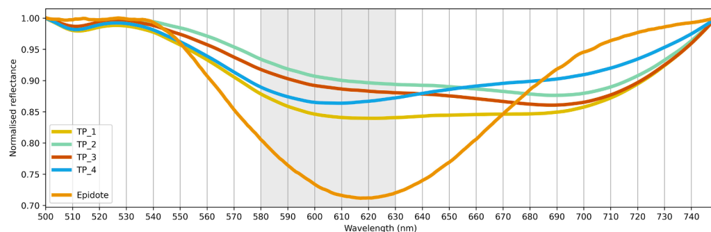
Fig. 16. Average hull normalised spectra from Tropicana domains. The spectrum of epidote (Kokaly et al., 2017) is provided as a reference for the identified 605 \pm 25 nm feature within TP_4.
