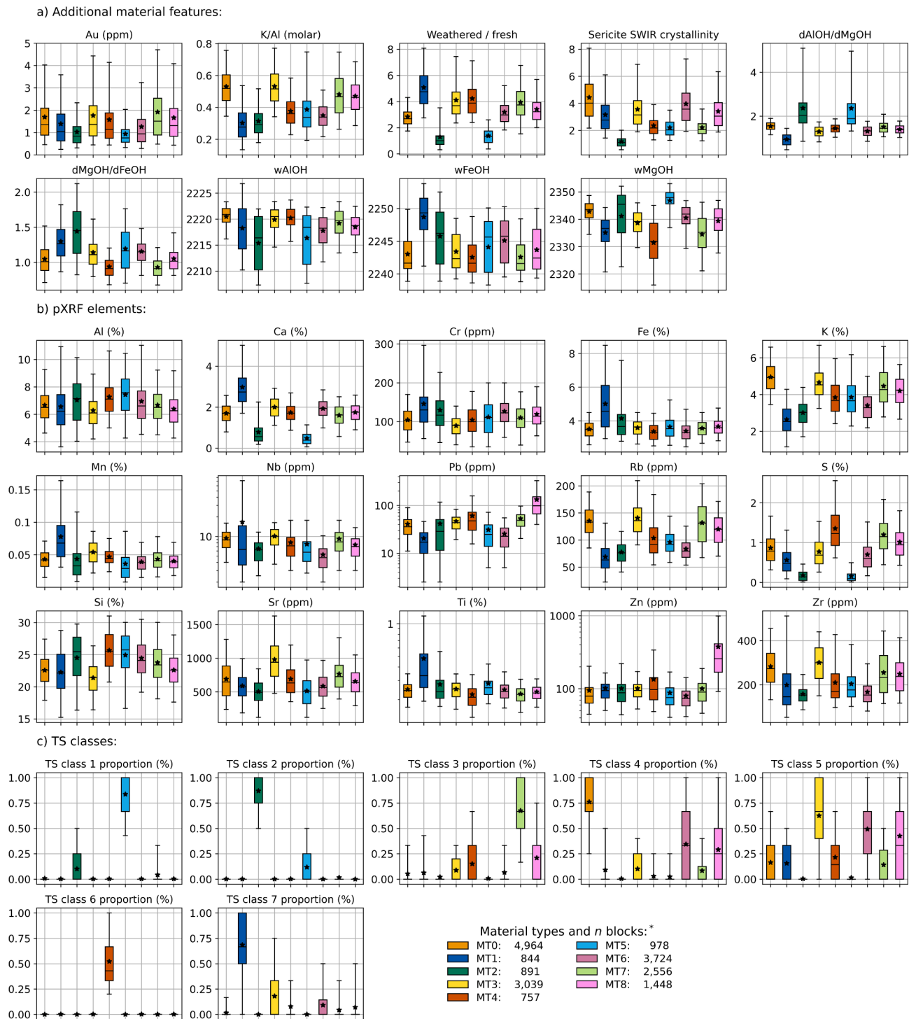
Fig. 11. Box and whisker plots of attributes of the block feature clustering blocks ( n = 19,201 ); (a) Interpreted material features; (b) pXRF elemental concentrations; (c) TerraSpec (TS) classes. *The n blocks for part (a) are less as not all parameters are acquired for all blocks.
