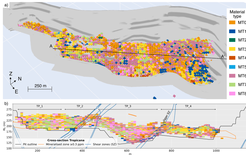
Fig. 12. Block model ( 12 \times 12 \times 3 m blocks) blocks coloured by material type class label; (a) oblique view of the Tropicana pit displaying the pit outline in light grey; (b) SW–NE 50 m thick cross-section along line A–A'.
