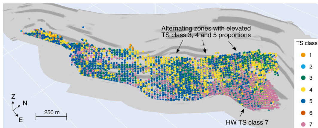
Fig. 9. Oblique view of the Tropicana pit displaying the pit outline in light grey with samples ( n = 46,485) coloured by TS class. Alternating zones occur in SW to NE direction and by depth. HW: hanging wall.
