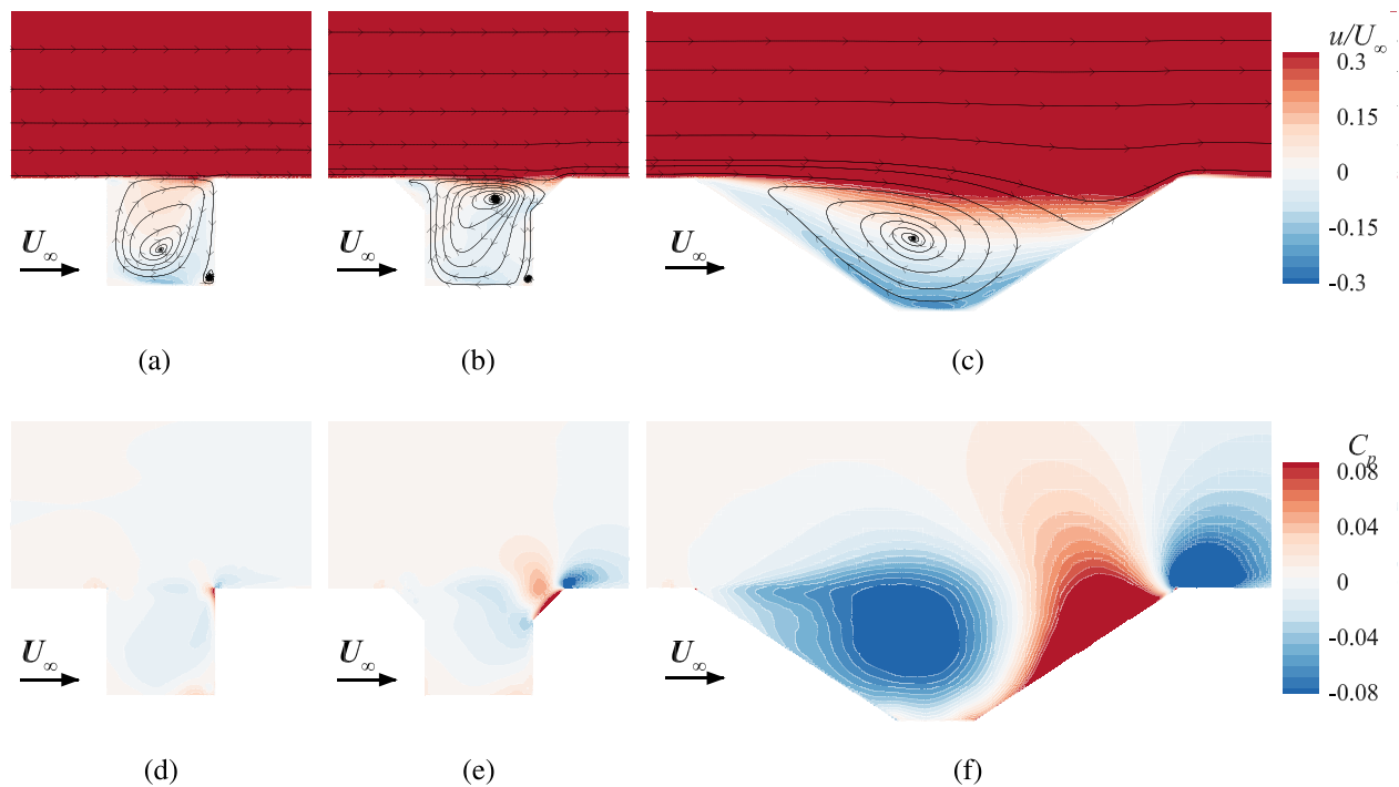
FIG. 11. Uncovered cavities average flowfield, located at the z=0 plane (center of the cavities). Streamwise velocity contours and in-plane streamtraces: (a) cylindrical, (b) countersunk, and (c) conical. Pressure coefficient contours: (d) cylindrical, (e) countersunk, and (f) conical.
