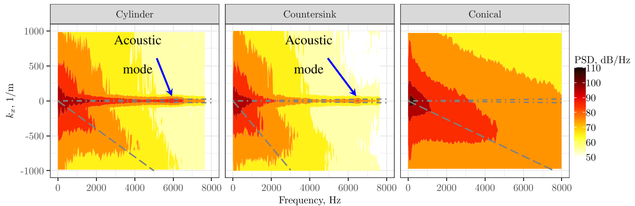
FIG. 15. Wavenumber-frequency spectra across the bottom of the uncovered cavities (dashed lines) lines represent the hydrodynamic peak due to recirculation, (dashed dotted lines) represents the area between the acoustic region. p_{\text{ref}} = 2.0 \times 10^{-5} Pa.
