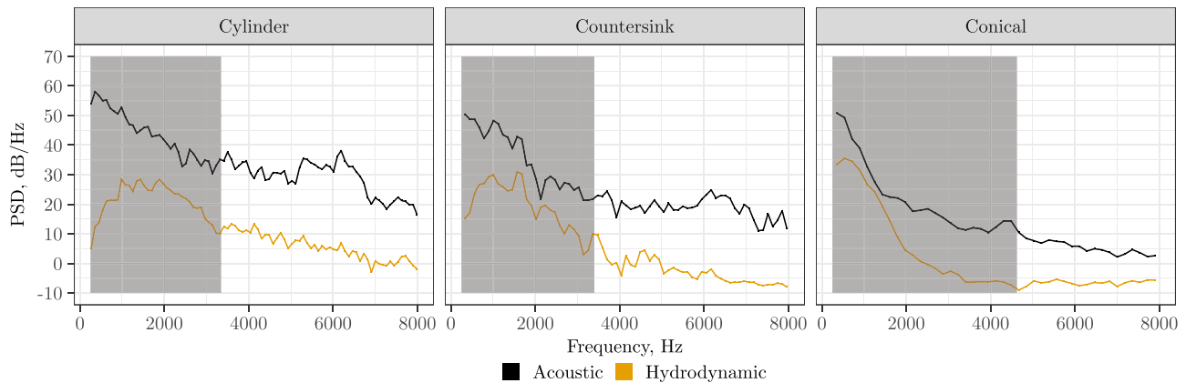
FIG. 20. Decomposition of the wavenumber spectra into acoustic and hydrodynamic components for all three covered cavities. Shaded area is the region of uncertainty.
