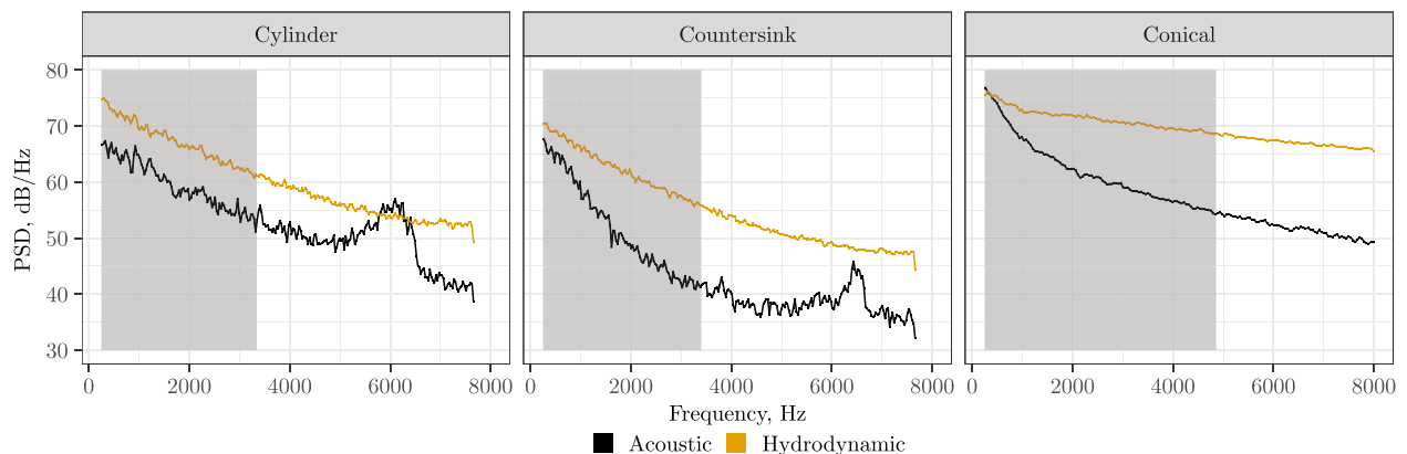
FIG. 16. Wavenumber spectra decomposed into acoustic and hydrodynamic components for all three uncovered cavities. Shaded area is the region of uncertainty, defined as f \leq U_\infty \Delta k .
