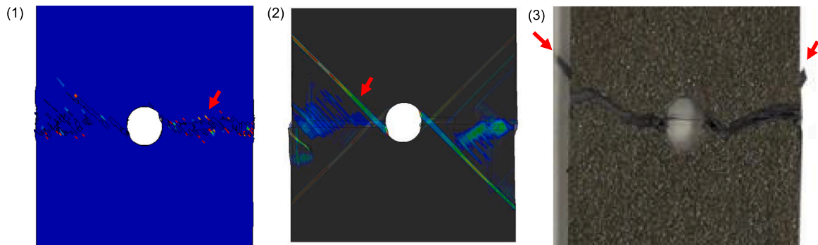
Fig. 15. Detailed look at failure mode of [50/40/10] open-hole tension analysis: (1) CDM3D , compressive fiber failure within matrix splits; (2) CDM-LD , large shear deformation (5%–50%) at the local scale within fully developed matrix splits; (3) Indication of ply splits in published experimental failure mode open-hole, adapted from Falcó et al. [16].
