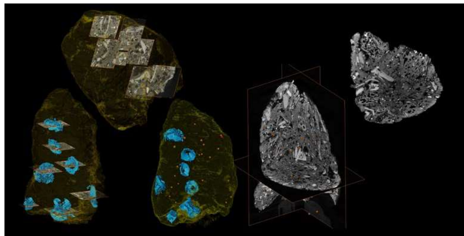
Figure V.3 S3-2, scan 0.040 mm voxel. Distribution of vertebrae and pike teeth in coprolite S3-2. Orange dots point at teeth. Note also the large 4 to 5 mm high cavernous bones (right).
