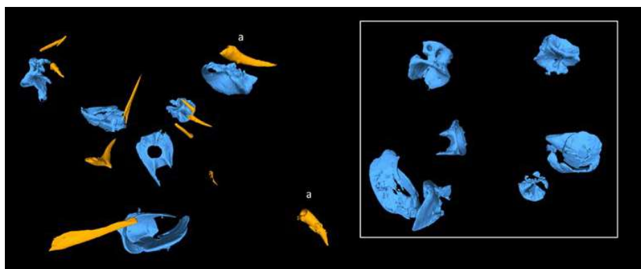
Figure V.15 S3-20, sub-scan 0.010 mm voxel. 6 vertebrae (blue) and pointed bones (orange); among them, several pike teeth (a). The verso side of the 6 vertebrae is framed on the right; the top right vertebra belongs to a cyprinid fish.
