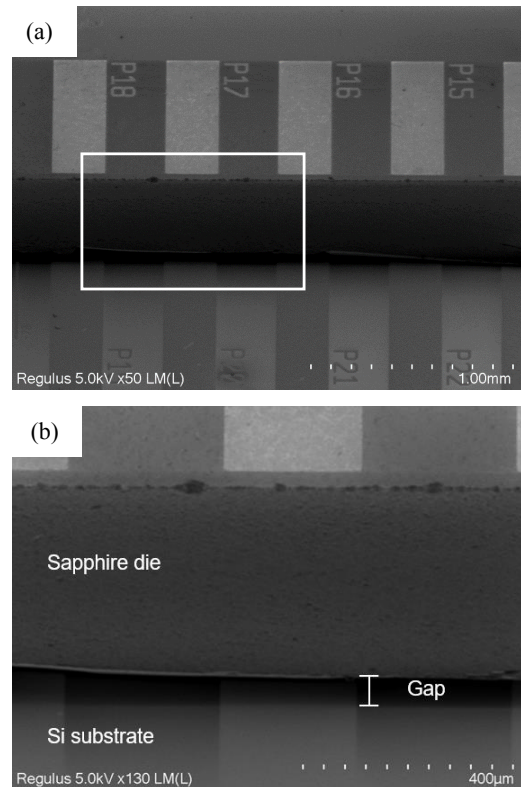
Fig. 5. (a) SEM image of the bonding edge at a 45° tilt angle. (b) Close-up view of the side-edge, indicated by the white box in (a), showing the alignment result and the gap due to Cu bumps.
