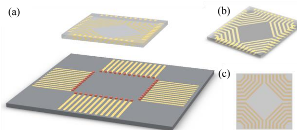
Fig. 1. Schematic illustration of (a) 3D stacked structure of sapphire chip to Si substrate nano-Cu joints flip chip, (b) flipped sapphire chip with Au deposition patterns and (c) the front side of sapphire chip with the Au interconnect lines.
