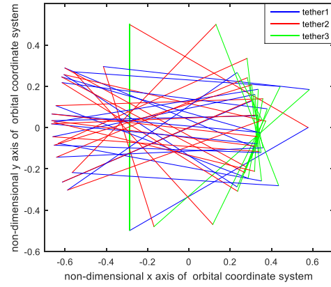
Fig. 3. System formation when \theta' = 0.5 .
