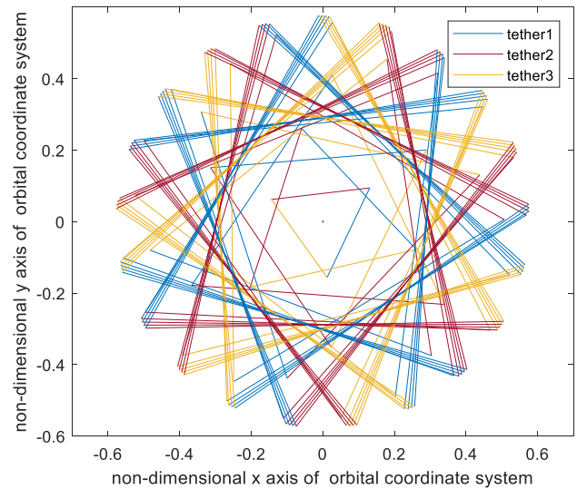
Fig. 13. Tethered triangle formation in simple version.
