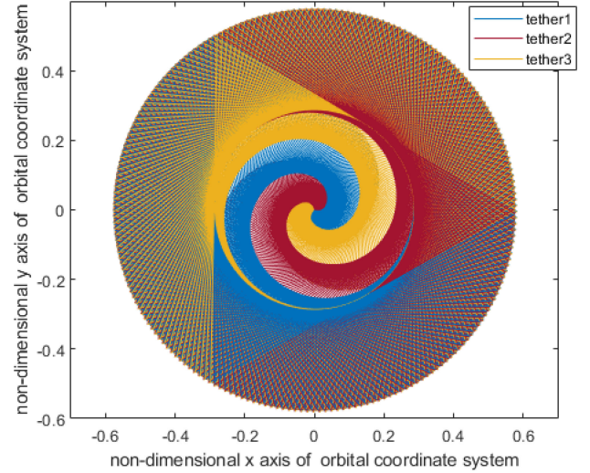
Fig. 12. Tethered triangle formation in full print version.
