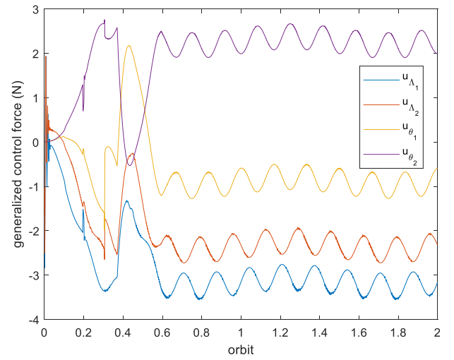
Fig. 11. Generalized control forces.
