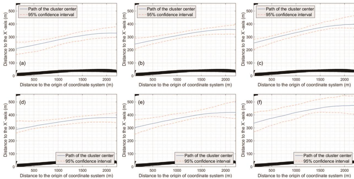
Figure 3.4. Clustered inbound ship paths: (a) cluster #1; (b) cluster #2; (c) cluster #3; (d) cluster #4; (e) cluster #5; (f) cluster #6 (The distance to the X' -axis as a function of the distance to the origin of the coordinate system with the sailing direction from the left to the right of the figure). The black bar at the bottom of each plot indicates the mole, Splitsingsdam, as shown in Figure 3.1.
