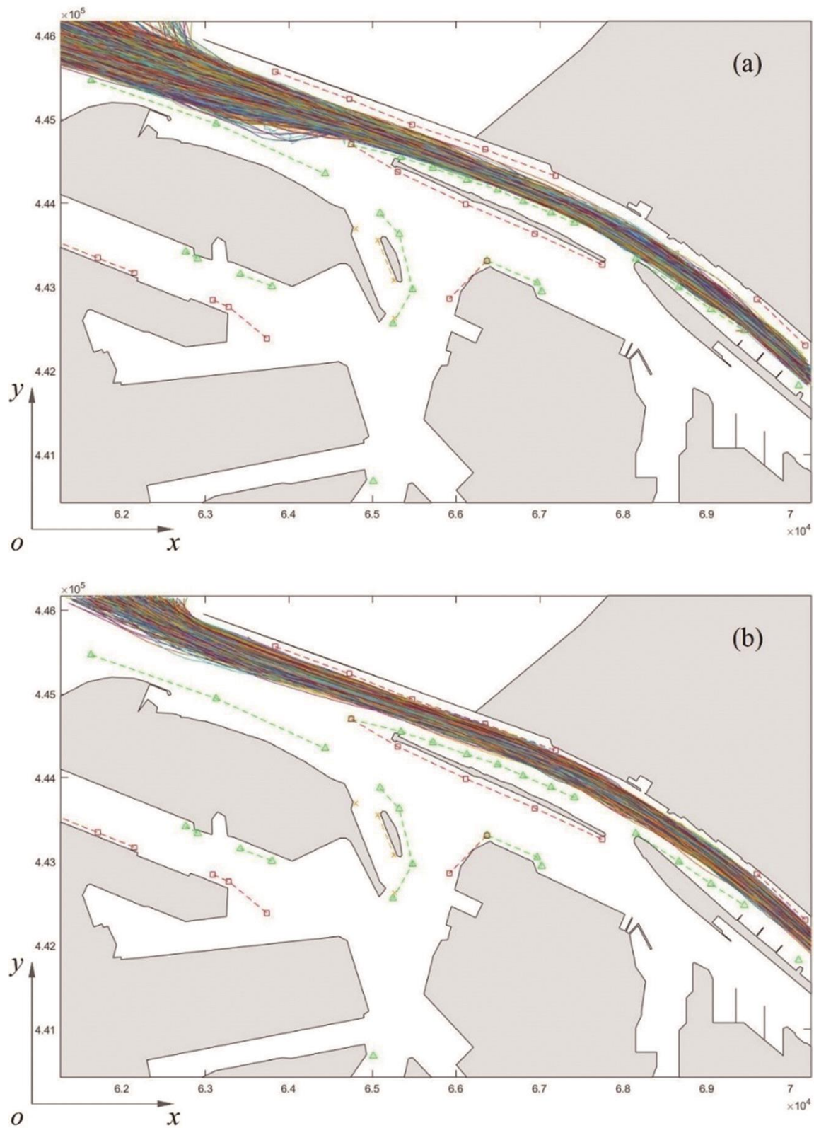
Figure 4.2. Overview of trajectories without any encounter of other ships in AIS data (The o-xy coordinate system is RD system.): (a) inbound 4051 trajectories by 738,667 messages; (b) outbound 4746 trajectories by 683,071 messages.
