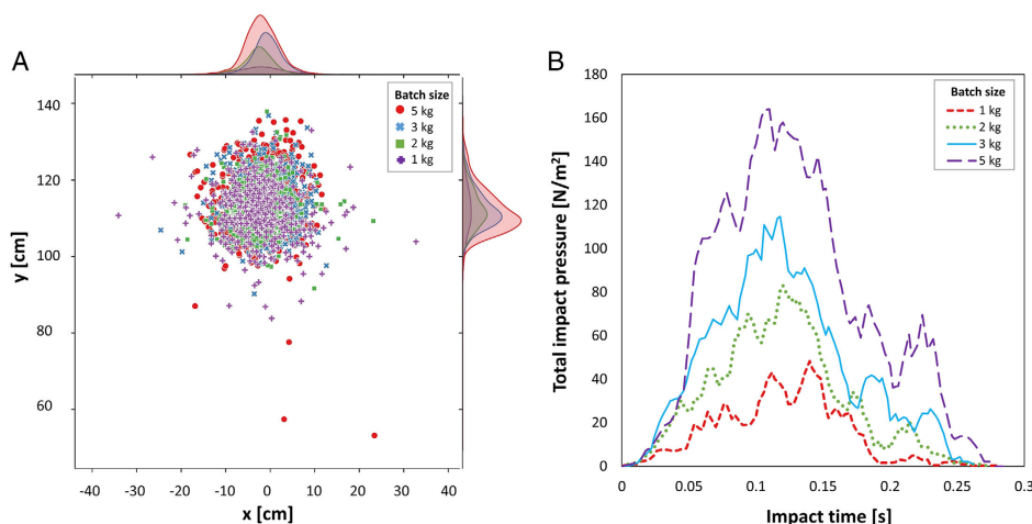
Figure 12. A) Effect of batch size on particle position and B) impact pressure for inclination 20°: bottom valve.
