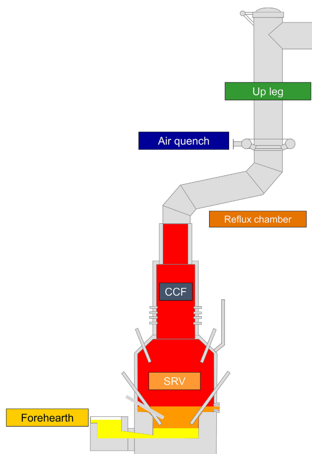
Figure 1. Schematic overview of the HIsarna pilot reactor, including off-gas system.
