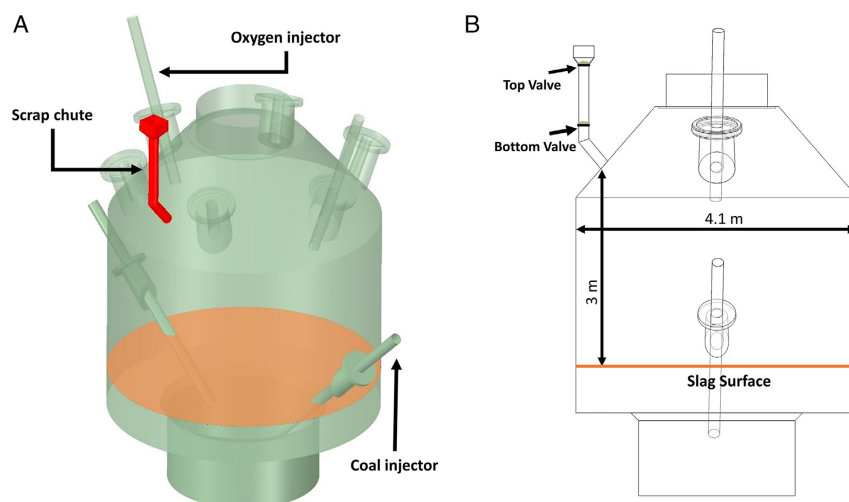
Figure 2. Schematic view of SRV and dimension used for simulations.
