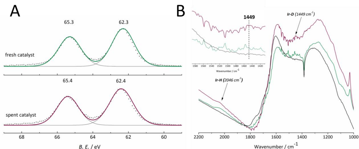
Figure 3.5. A) Iridium 4f XPS spectra of the 16 wt% loaded catalyst, before (green, top) and after (red, bottom) use B) DRIFT spectra of the pure CTF (black) 16 wt.% Ir loaded (green), and 16 wt.% in the experiment with deuterated formic acid (red).
