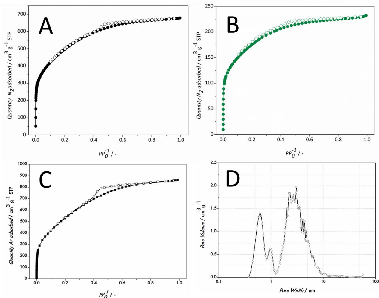
Figure 3.3. Nitrogen adsorption isotherms for A) mesoporous CTF support and B) Ir@CTF catalyst with Ir loading of 16 wt%. C) Argon adsorption isotherm of CTF D) DFT calculated Pore size distribution of CTF.
