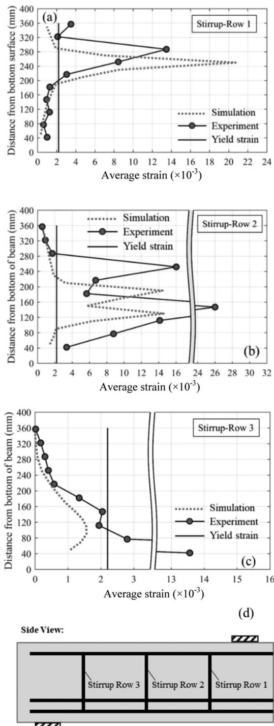
FIGURE 30 Strain distribution along stirrups at the peak load: (a) first row; (b) second row; (c) third row; and (d) schematic representation of reinforcement position
