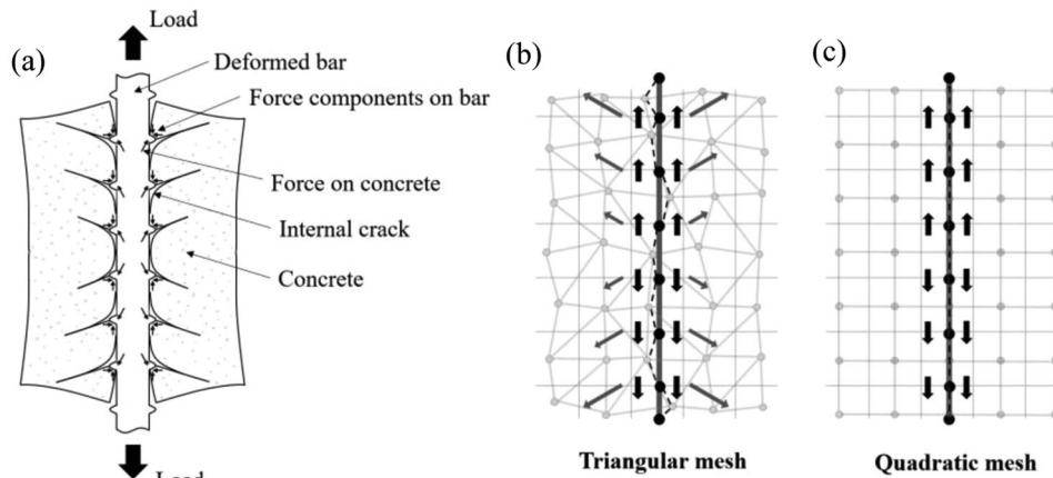
FIGURE 21 Schematic diagram for bond stress transfer mechanism of reinforcement in concrete: (a) internal cracks around the deformed bar and stress transfer mechanism based on the (b) triangular mesh, and (c) regular quadratic mesh
