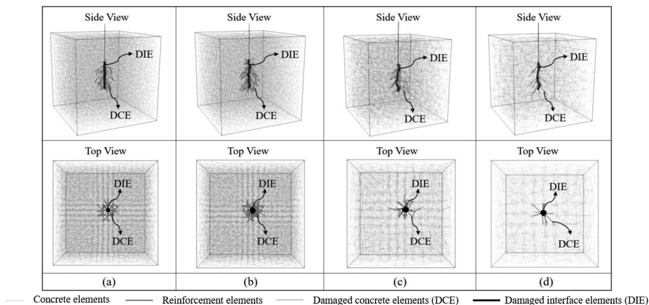
FIGURE 15 Damage pattern at a slip of 3.0 mm for one-end reinforcement pull-out: (a) aligned interface elements with mesh of 10 mm, Input 1; (b) non-aligned interface elements with mesh of 10 mm, Input 2; (c) non-aligned interface elements with mesh of 15 mm; and (d) non-aligned interface elements with mesh of 20 mm
