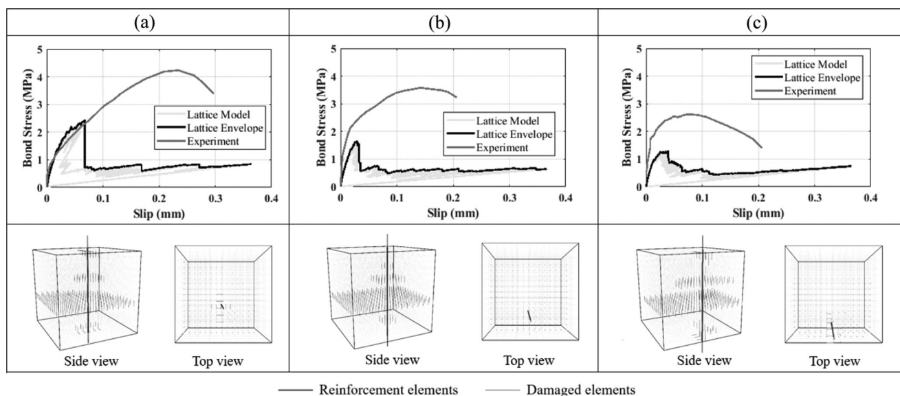
FIGURE 20 Simulated bond stress-slip relationship and crack pattern at peak load for the quadratic mesh: (a) concrete cover of 50 mm; (b) concrete cover of 30 mm; and (c) concrete cover of 10 mm
