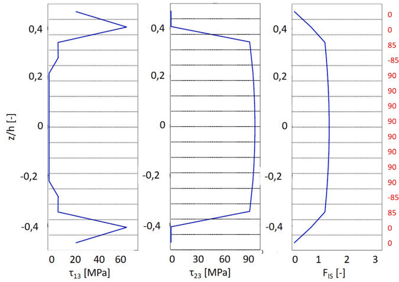
Fig. 2. Characteristics of the optimal non-constrained laminate. Through-thickness distributions of interlaminar stresses \tau_{13} (left), \tau_{23} (middle), interlaminar stress function f_{IS} (right).
