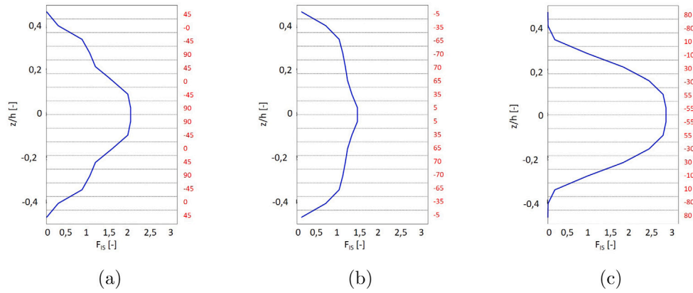
Fig. 3. Through the thickness distribution of f_{IS} in several laminates: (a) reference laminate, [45/0/-45/90]_{2s} , ( \max(f_{IS}) = 2.05 ); (b) best optimum dispersed-ply laminate, B1: [-5/-35/-65/-70/70/65/35/5]_s , ( \max(f_{IS}) = 1.47 ); (c) non-optimal dispersed-ply laminate with lower performance than the reference, [80/-80/10/-10/30/-30/55/-55]_s , ( \max(f_{IS}) = 2.89 ).
