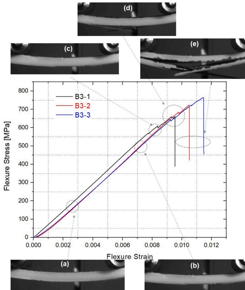
Fig. 7. Four-point bending test for “B3” laminate [-5/-45/-45/90/90/45/45/5]_s .
