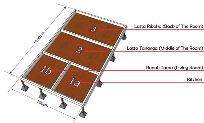
Figure 4. Floor plan of Ammatoa community's houses.
