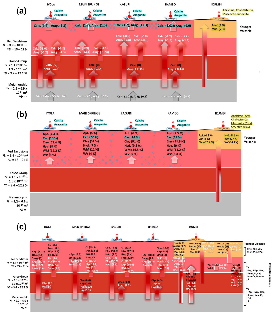
Fig. 11 The scheme of water–rock interaction for surface thermal springs ( a and b ) and for estimated reservoir water ( c and d ) at 125 °C (black ink) and 148 °C (white ink) when reacting with different lithology in the Songwe geothermal area. Lithologies are shown in different colors including porosity and permeability values. Arrows show the reaction pathway, covering the reaction with 1–3 layers and resulting saturation indices. The highlighted minerals in blue correlate with the highlighted minerals at surface of each thermal spring. a model outputs only focusing on calcite (calc.) and aragonite (arag.); it suggests the thermal springs are only in contact with Red Sandstone, and Ikumbi is also in contact with metamorphic rocks, Karoo
