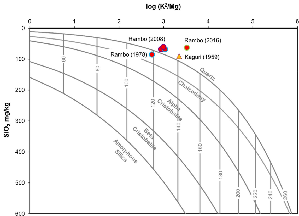
Fig. 7 Diagram of SiO 2 versus log K 2 /Mg of Songwe thermal water, concentration in mg/l, based on Giggenbach and Soto (1992). The curves provide information on equilibrium attainment for SiO 2 and K–Mg geothermometers. Most thermal water plots near the quartz
