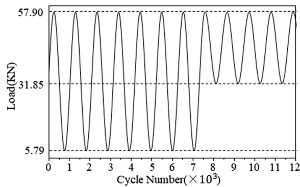
Figure 3. The load spectrum and beach mark generating procedure.
