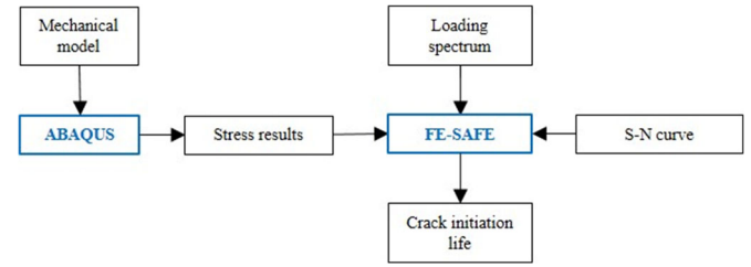
Figure 8. Flowchart of combining ABAQUS and FE-SAFE to evaluate the crack initiation life [31].
