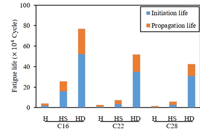
Figure 21. Numerical results of the fatigue life of all FE models.
