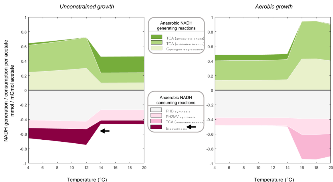
Fig. 3. Balance and reactions involved in the NADH generation (green) and consumption (magenta) during the anaerobic phase at different temperatures of the unconstrained growth (left panel) model and the aerobic growth (right panel) model. Black arrow indicates the use of NADH for biosynthetic reactions showcasing the main difference in the structure between both models. Biosynthesis comprised all reactions synthesizing enzymes, ribosomes and biomass precursors. For the specific reaction stoichiometry, please see Table S1. Abbreviations: tricarboxylic acid cycle (TCA), poly-hydroxy-butyrate (PHB), poly-hydroxy-2-methylvalerate (PH2MV).
