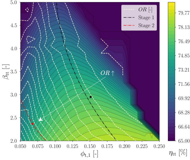
FIGURE 2: Design map of \eta_{tt} and OR computed for R1233zd(E) at P_{t1} = 0.5 bar, T_{t1} = 283.15 , \psi_{is} = 0.8 . The dashed black and red lines correspond to the theoretical locii of optimal design for the two stages, computed by maximizing \eta_{tt} of stage 1 and fixing \psi|_{s1}/\psi|_{s2} = 1 . The black and red dots correspond to the design point selected by the multi-objective optimizer.
