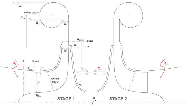
FIGURE 3: Meridional view of a centrifugal compressor, featuring two stages mounted in back-to-back configuration on the same shaft.
