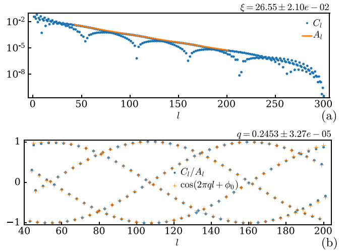
FIG. 5. Demonstration of the two-step fitting scheme for a 601 site simulation along the c_8 cut, at (\Delta/\Omega, \mathcal{R}_b) = (2.23, 3.32) .
