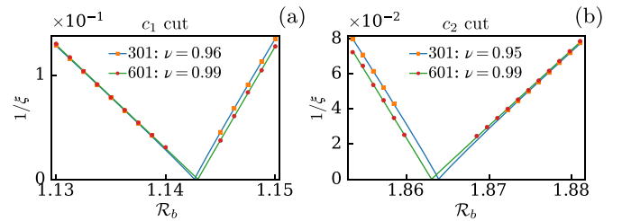
FIG. 6. Correlation length along the \Delta/\Omega = 3 cut (a) that crosses the commensurate transition line below the period-2 lobe, and the \Delta/\Omega = 2 cut (b) that crosses it above. All points shown in the disordered sides are inside the commensurate phase. The small finite-size effects observed let us conclude from the exponent obtained that the transition is in the Ising universality class.
