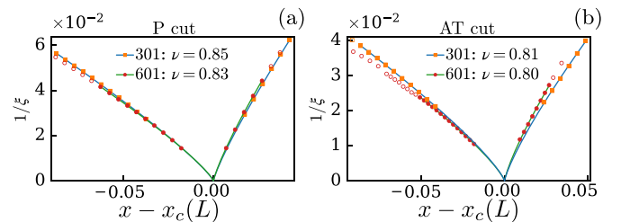
FIG. 12. Inverse correlation length along the p = 3, 4 conformal cuts, as a function of the parametric distance to the estimated critical points ( x \equiv \Omega/\Delta ).
