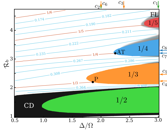
FIG. 2. Phase diagram of the Rydberg model obtained with DMRG simulations on 121 sites. Red, blue, orange, and green regions are the ordered phases with period p = 5, 4, 3 , and 2 , respectively, while the black region is a commensurate disordered (CD) phase with wave vector q = 1/2 in units of 2\pi . The gray region is a sketch of the floating phase based on a previous iDMRG work [19]. Equal- q lines are shown in the disordered and floating phases. The points P and AT are, respectively, our estimates of the Potts and Ashkin-Teller critical points. Apart from the cuts that go through these points, either horizontally or vertically, or along the associated commensurate lines (P and AT cuts), the other cuts discussed throughout the text are horizontal or vertical and are labeled c_n . They are represented by arrows colored according to the ordered phase they cross.
