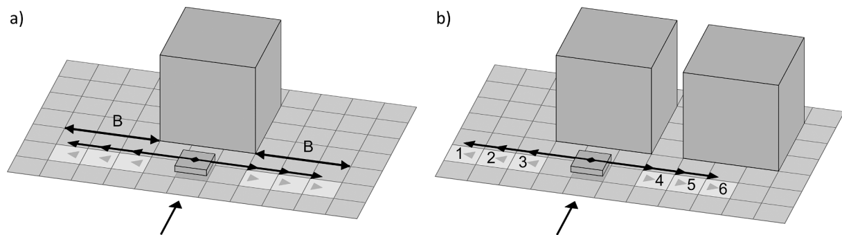
Fig. 15. A slab in transport upwind of a building. If this slab is moved sideward, it is shifted to a random cell in of the destination area, i.e. the lighter coloured cells of the same grid row (the same distance upwind of the building), at between 1 cell and a distance B to the side of the building. Cell numbers are referred to in the text.
