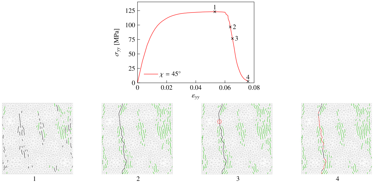
Fig. 23. Evolution of microcracking process after the material strength is reached (snapshot 1); gray color indicates uncracked element boundaries, green color stand for unloading cohesive segments, black color indicates damaging but not completely broken cohesive segments, red color represents formed microcrack with zero cohesive traction.
