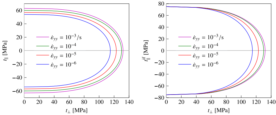
Fig. 11. Microcrack initiation envelopes for matrix (left) and matrix/fiber interface (right) for different strain-rates, according to Eq. (66).
