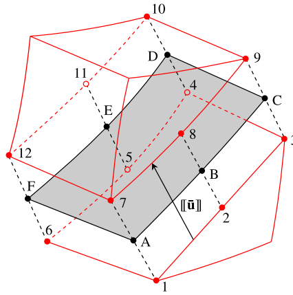
Fig. 5. Wedge-shaped bulk finite elements in decohesion process defined by displacement jump \llbracket \mathbf{u} \rrbracket ; cohesive segment represented as mid-surface between the two bulk elements.
