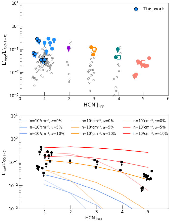
Fig. 10. Comparison of L'_{\text{HCN}(1-0)}/L'_{\text{CO}(1-0)} ratios in DSFGs for HCN(1–0) to (5–4) observations from the literature ( upper ). The coloured points indicate high- z measurements; grey ones z = 0 observations. Our HCN(1–0) measurements are outlined in black; the star indicates the limit from the stacked K-band spectrum. Lower : high- z HCN measurements, compared to the predictions of PDR models from Kazandjian et al. (2015). We vary the PDR gas density ( n = 10^3 – 10^5 \text{ cm}^{-3} ) and the mechanical heating factor ( \alpha = 0 – 10\% ). The FUV irradiation is fixed to G = 10^4 G_0 . The current high- z HCN detections can not be reproduced by models with n \leq 10^4 \text{ cm}^{-3} without significant mechanical heating. High- z data: HCN(1–0): Carilli et al. (2005), Gao et al. (2007), Oteo et al. (2017); HCN(2–1): G. Jolink (BSc thesis); HCN(3–2): Danielson et al. (2013), Oteo et al. (2017); HCN(4–3) and (5–4): Béthermin et al. (2018), Cañameras et al. (2021). Low- z data: HCN(1–0): Gao & Solomon (2004b), García-Burillo et al. (2012); HCN(2–1): Krips et al. (2008), HCN(3–2): Bussmann et al. (2008), Li et al. (2020), HCN(4–3): Zhang et al. (2014). The squares correspond to the Spilker et al. (2014) stacking analysis.
