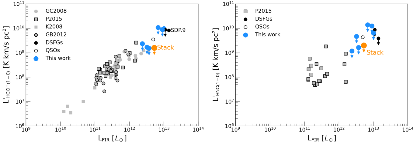
Fig. 6. As Fig. 5, but for \text{HCO}^+(1-0) and \text{HNC}(1-0) . Notice the increased scatter compared to the FIR-HCN relation and the paucity of observations at high redshift.
