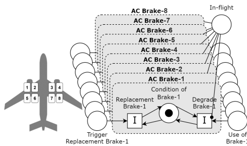
Fig. 5. SDCPN model for the landing gear brakes of a wide-body aircraft.
