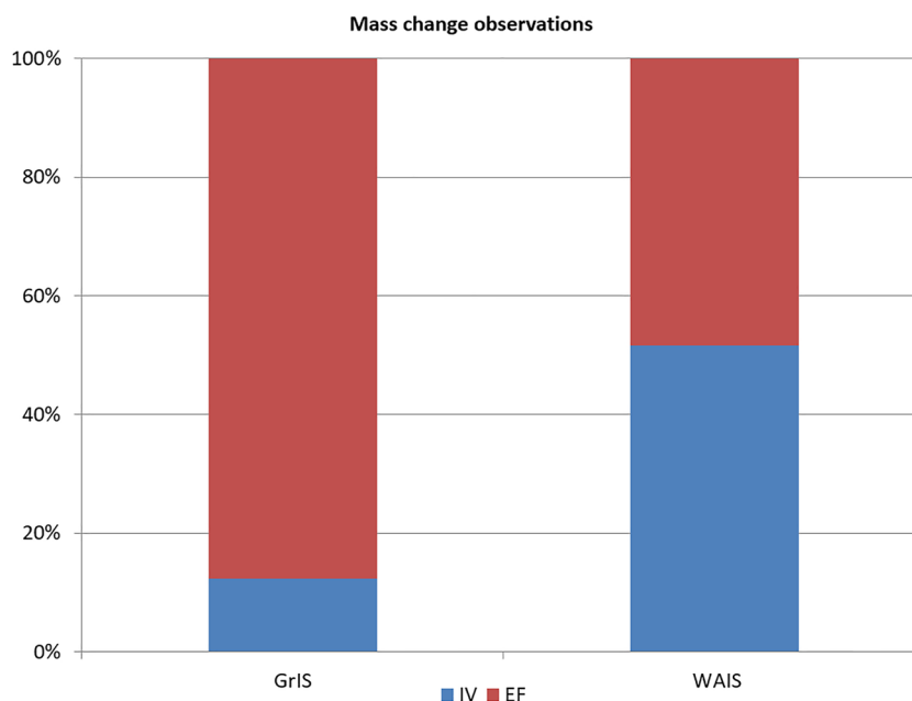
Figure 5. Expert judgements for whether internal variability (IV) or external forcing (EF) is the dominant driver of recent (last two decade) observational trends in mass balance for the Greenland Antarctic ice sheets (GrIS) and West Antarctic Ice Sheet (WAIS).
