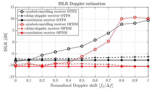
Fig. 3. Integrated side-lobe ratio in the Doppler estimation for f_d \leq \Delta f . N = 8 and M = 10 .
