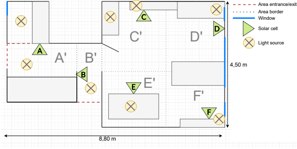
(a) Layout of the evaluation area.
