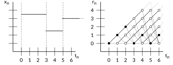
Figure 8: Evolution of the value for run length r_n for a signal x_n with changepoints at t=3 and t=5 . Left: The data point received at each timestep. Right: The evolution of the run length r_n . For each timestep, the value of r_n increases by one (solid line), or it is reset to r_n = 0 when a changepoint occurs (dashed line). The value of r_n that is most likely for the timestep is colored black.
