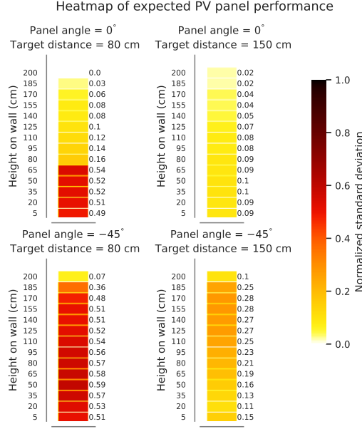
Figure 3: Heatmap
