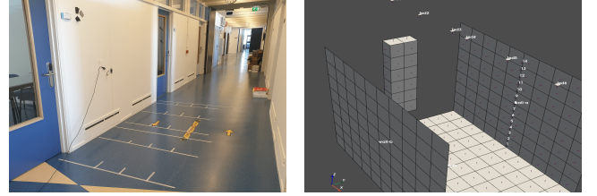
(a) Picture of the hallway during the experiments (with only one solar cell). (b) Screenshot of the hallway in simulation.
