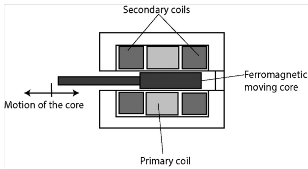
Figure 1. The basic principle of LVDT transducer.
