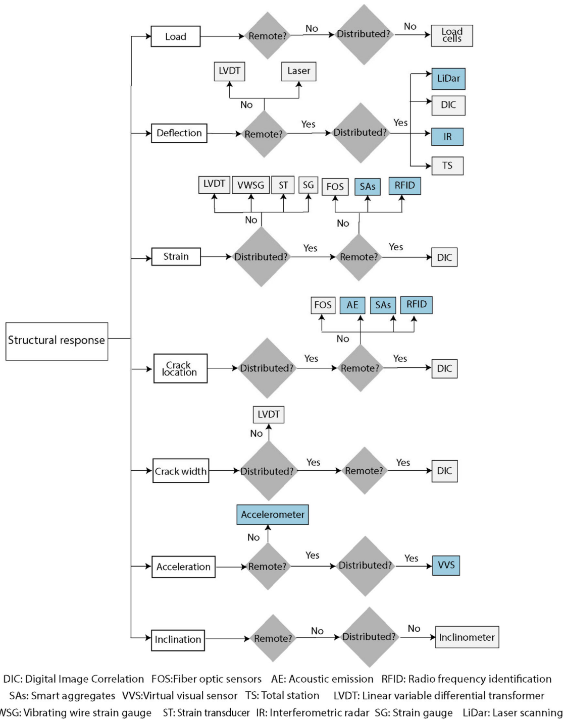
Figure 27. Measuring technique or sensor selection flow chart.
