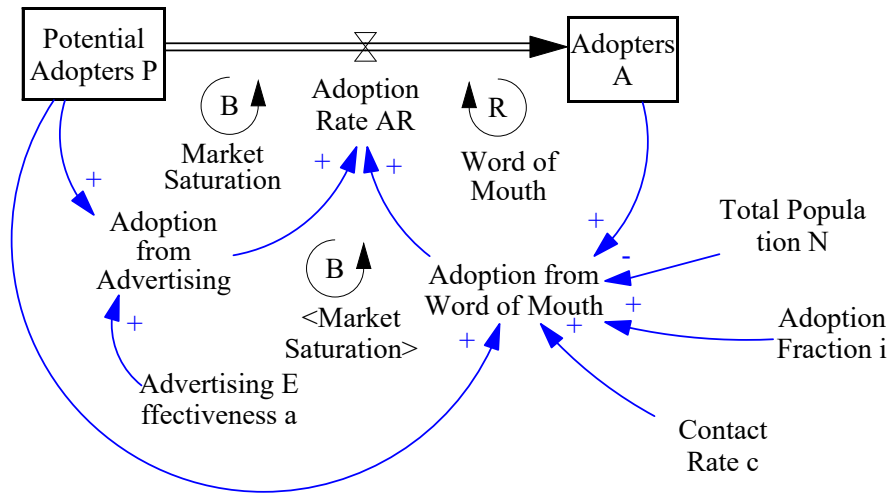
FIG. 6.1 SFD of the Bass Diffusion model developed by (Stermann, 2000)
