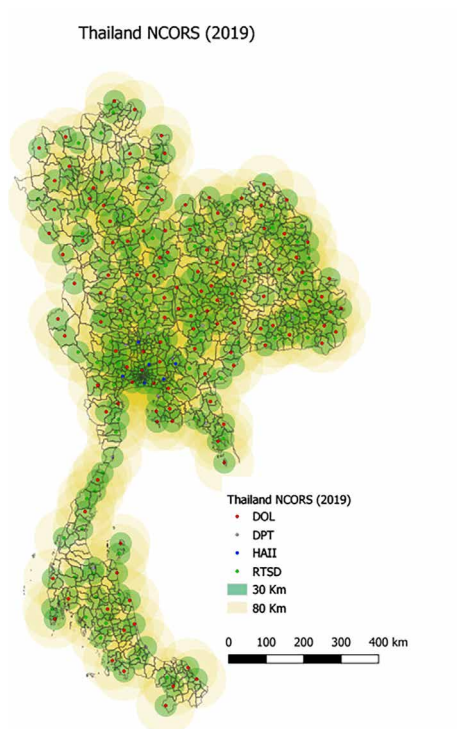
FIG. 4.17 The distribution and densification of CORS providers in Thailand NCORS (Source: the author)
