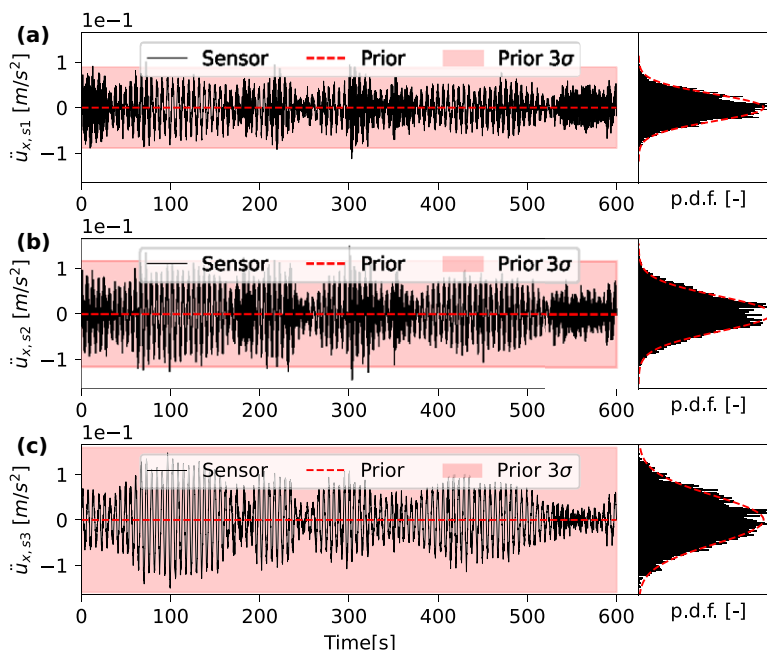
Figure 7. Record PK1-x. Prior distribution visual check using optimum hyperparameters: l_{sc} = 0.318 s, \sigma = 2556 N. (a) Sensor s1. (b) Sensor s2. (c) Sensor s3.
