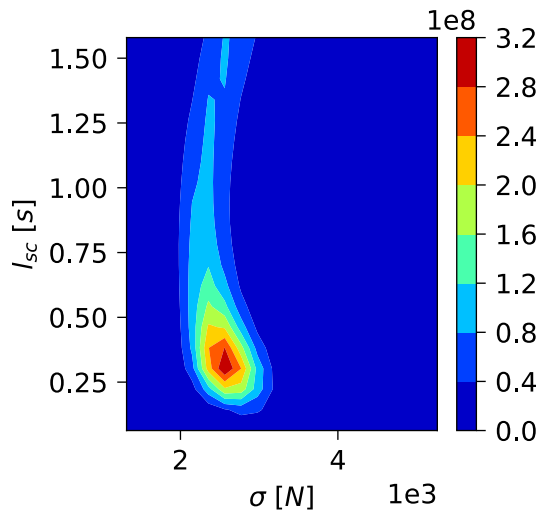
Figure 6. Record PK1-x. \sigma and l_{sc} estimation. Objective function plot: q_{s1,s2,s3} . Optimum found for maximum value: l_{sc} = 0.318 s, \sigma = 2556 N.
