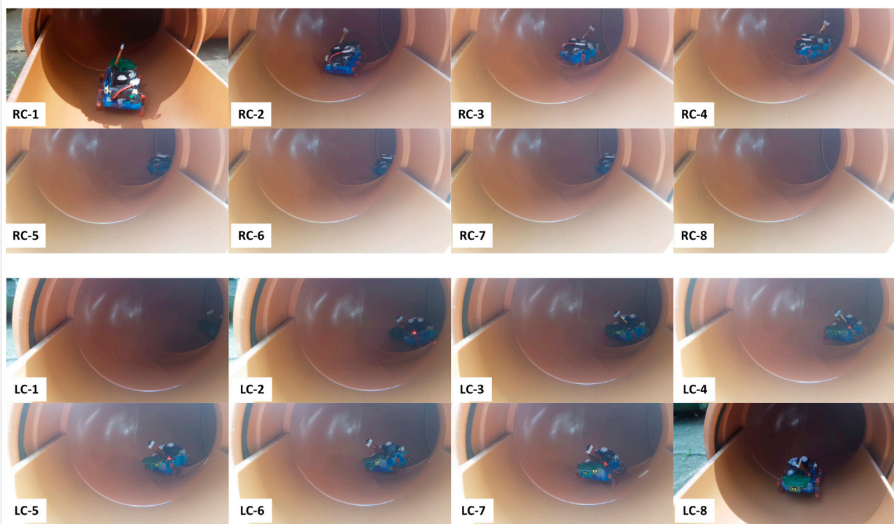
FIGURE 8 Successful detection, decision making and maneuvers of the Joey robot at right (RC-1 to RC-8, top two rows) and left (LC-1 to LC-8, bottom two rows) corners during autonomous pipe exploration.
