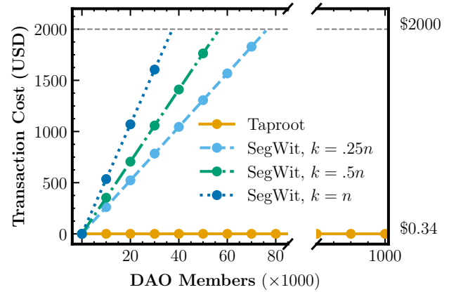
Figure 4: Transaction costs for governance decisions using the Bitcoin blockchain.
