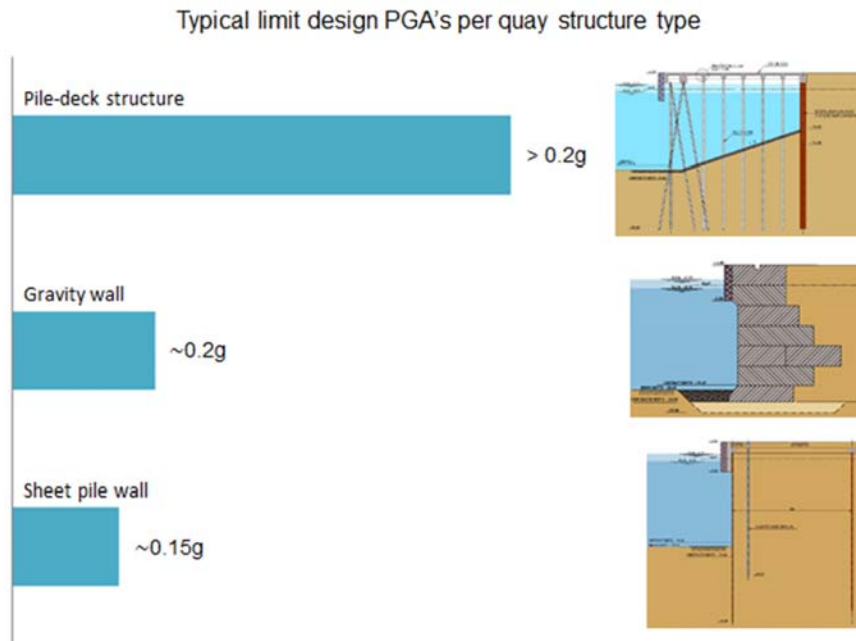
Fig. 1 Observed trend in seismic quay design [3]
