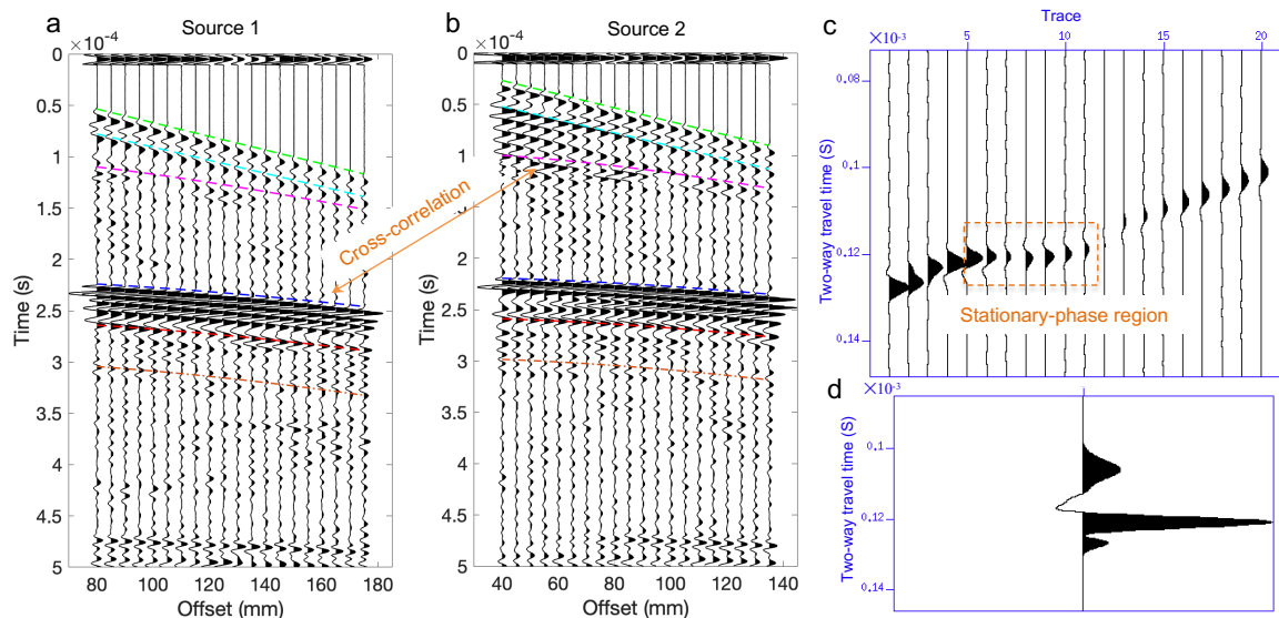
Figure 3 (a) Common-source gather from Source 1. Arrivals are indicated using the colour-coding from Figure 2a: green for the direct wave, cyan for the refracted wave, magenta for the P-wave reflected from the mud top, blue for the P-wave reflected from the mud bottom (PPPP), red for the P-to-S conversion at the mud bottom (PPSP), and orange for the P-to-S at the water/mud interface (PSSP). (b) Common-source gather from Source 2 with the same color-coding. (c) Correlation panel for retrieval of a ghost reflection inside the mud layer obtained by correlating the magenta reflection in b with the blue PPPP reflection in a. The orange rectangle indicates the stationary-phase region. (d) The result of stacking the traces in the correlation panel in c.
