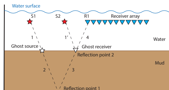
Figure 1 Application of seismic interferometry by cross-correlation in fluid-mud reflection tests. The two red pentagrams represent the seismic sources, S1 and S2. The blue triangles are the receiver array with the left-most receiver labelled R1. The white pentagram and triangle represent the ghost source
