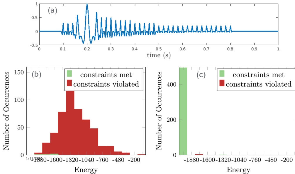
Figure 1 (a) input trace for the simple synthetic, (b) QPU output histogram without and (c) with post-processing.
