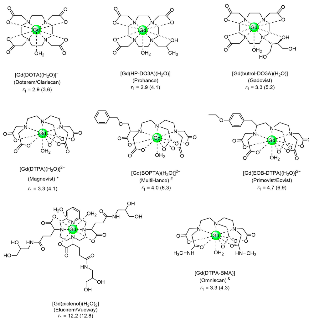
Figure 1. Schematic representation of the molecular structure of commercial Gd-based contrast agents. Relaxivities are in s -1 mM -1 at 1.5 T and 310 K in aqueous solutions and in biological medium (in brackets). Charges are omitted for clarity. The brand names are given between brackets. * The European Medicines Agency (EMA) recommends restricting the use of this CA only for intra-articular use. # The EMA allows this CA only for liver scans. & Authorization suspended by the EMA.
