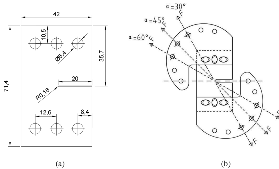
Fig. 11. Compact tension shear specimen and loading set-up [5].
