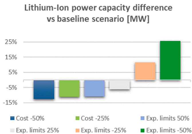
Fig. 11. Li-Ion sensitivity to DR parameters variation.
