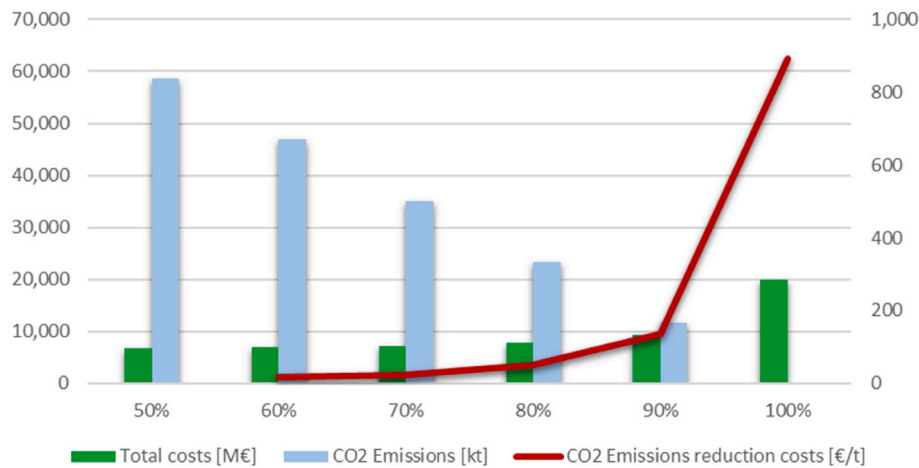
Fig. 10. Economic and environmental metrics under different decarbonisation objectives.
