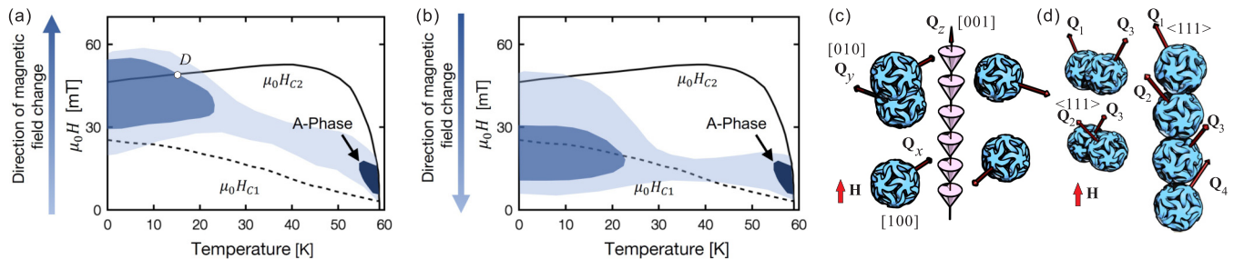
FIG. 1. Experimental phase diagrams indicating the extent and intensity of skyrmionic scattering after zero field cooling (ZFC) for \mathbf{H} \parallel [\mathbf{k}_f] \parallel [001] . The measurements were performed upon increasing the magnetic field (a) and decreasing the magnetic field (b). Deep dark blue stands for the high-temperature A-phase; dark blue—for the low-temperature SkL; and light blue—for the weak scattering that surrounds both the LT and HT skyrmion pockets and connects them. (c) Schematics showing coexisting helical domains with mutually orthogonal propagation directions (shown as blue balls). In an applied magnetic field, only the conical phase constitutes the energy minimum, whereas other spirals turn metastable. (d) Schematics showing coexisting domains of an oblique spiral tilting toward \langle 111 \rangle directions.
