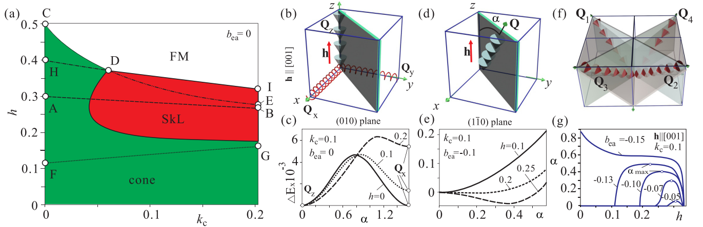
FIG. 2. (a) Phase diagram of the ground states derived from the model (2) for an applied magnetic field \mathbf{h} \parallel [001] and zero anisotropic exchange (1). The regions of the thermodynamical stability are colored red (skyrmions), green (cones), and white (saturated state). A-B and H-I are the lability lines of the spiral and skyrmion phases. C-D-E is the line of the first-order phase transition between the conical and the homogeneous states. At the dotted line F-G the energy of SkL becomes equal to the energy of the metastable helical spiral states with the wave vectors along the [100] and [010] directions. (b–g) Spiral reorientation for \mathbf{H} \parallel [001] . (b) Schematics of three spiral domains in low magnetic fields. At zero field, the spiral energy is degenerate with respect to the propagation vector. (c) Dependence of the spiral energy density on the wave vector \mathbf{Q} varying in the (010) plane at zero field and at h = 0.1; 0.2 . The global energy minimum is reached at \mathbf{Q}_z[001] immediately as the field is applied ( \alpha is given in radians). The local minimum corresponding to metastable spirals with their propagation perpendicular to the field persists up to relatively high field values. (d) Schematics of a tilted-spiral state that appears above a critical value of the magnetic field, in which \mathbf{Q} rotates away from the magnetic field vector toward the \langle 111 \rangle directions. (e) Energy density plotted as a function of the tilt angle \alpha in the (110) plane for several field values. (f) Schematics showing enumeration of wave vectors in the domains of a tilted spiral state. (g) Magnetic field dependence of the angle \alpha describing the tilt of the spiral wave vector \mathbf{Q} away from \mathbf{h} \parallel [001] toward the body diagonals for different values of |b_{ea}| . Above some critical value, \alpha increases from 0, which corresponds to the conical spiral phase, to a maximal value, \alpha_{\max} , and then decreases back to 0 as the magnetic field strength, h , increases. For b_{ea} > 0.14 , \mathbf{Q} \parallel \langle 111 \rangle even at zero field and smoothly rotates toward [001] with increasing field.
