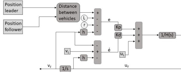
Fig. 4. Implementation of a CACC.
