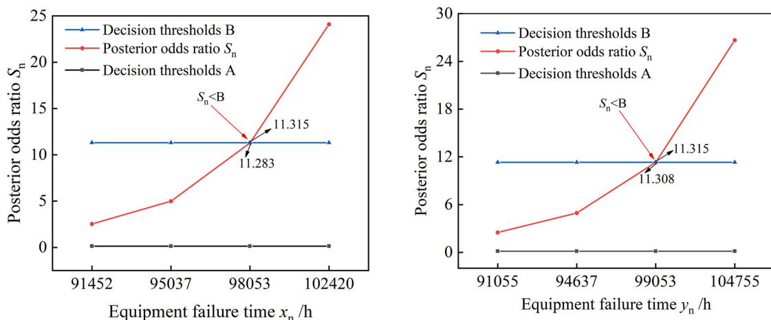
Fig. 5. Hypothesis testing results of x_n and y_n in RIUL method.
