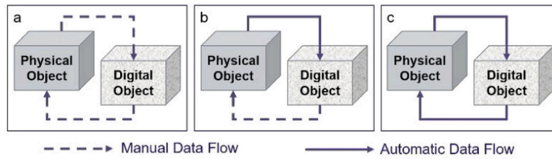
Fig. 4. Integration levels between virtual and physical environment for Digital Models (a.), Digital Shadows (b.), and Digital Twins (c.) Kritzing et al. (2018).
