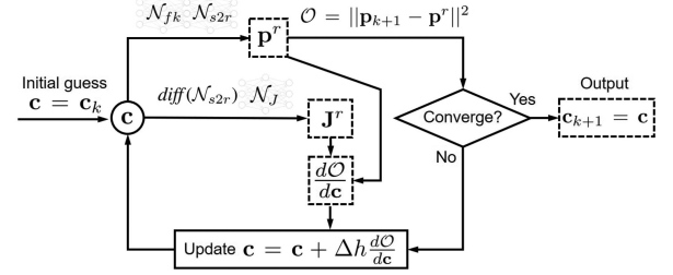
Fig. 1. Pipeline of the Jacobian-based method to determine the actuation parameters c_{k+1} for the waypoint p_{k+1} \in \mathcal{L} that solves the IK problem of soft robots by minimizing \mathcal{O}(\cdot) in (1). Both the position p^r in task space and the Jacobian J^r are effectively estimated by the networks N_{fk} , N_J , and N_{s2r} obtained from the offline training. When \mathcal{O} < \epsilon^2 , we regard the convergence as having been achieved (e.g., 0.1% of the workspace width is employed as \epsilon ).
