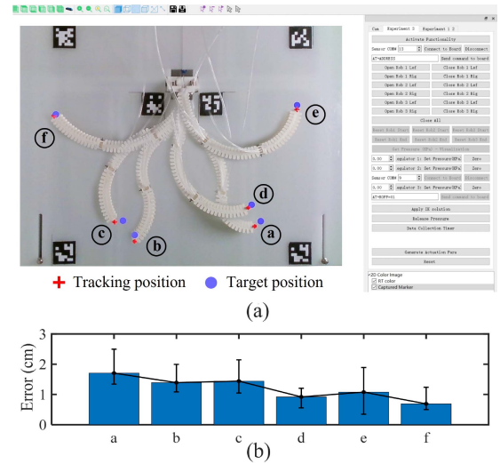
Fig. 13. Interactive positioning results for the soft manipulator with three finger actuators. (a) With a user-specified position given through the software interface, our Jacobian-based method is applied to determine the IK solution. (b) Bar chart presents the tracking errors for different target positions, where the repeatability is also studied and displayed as the range of deviation in tracking errors.
