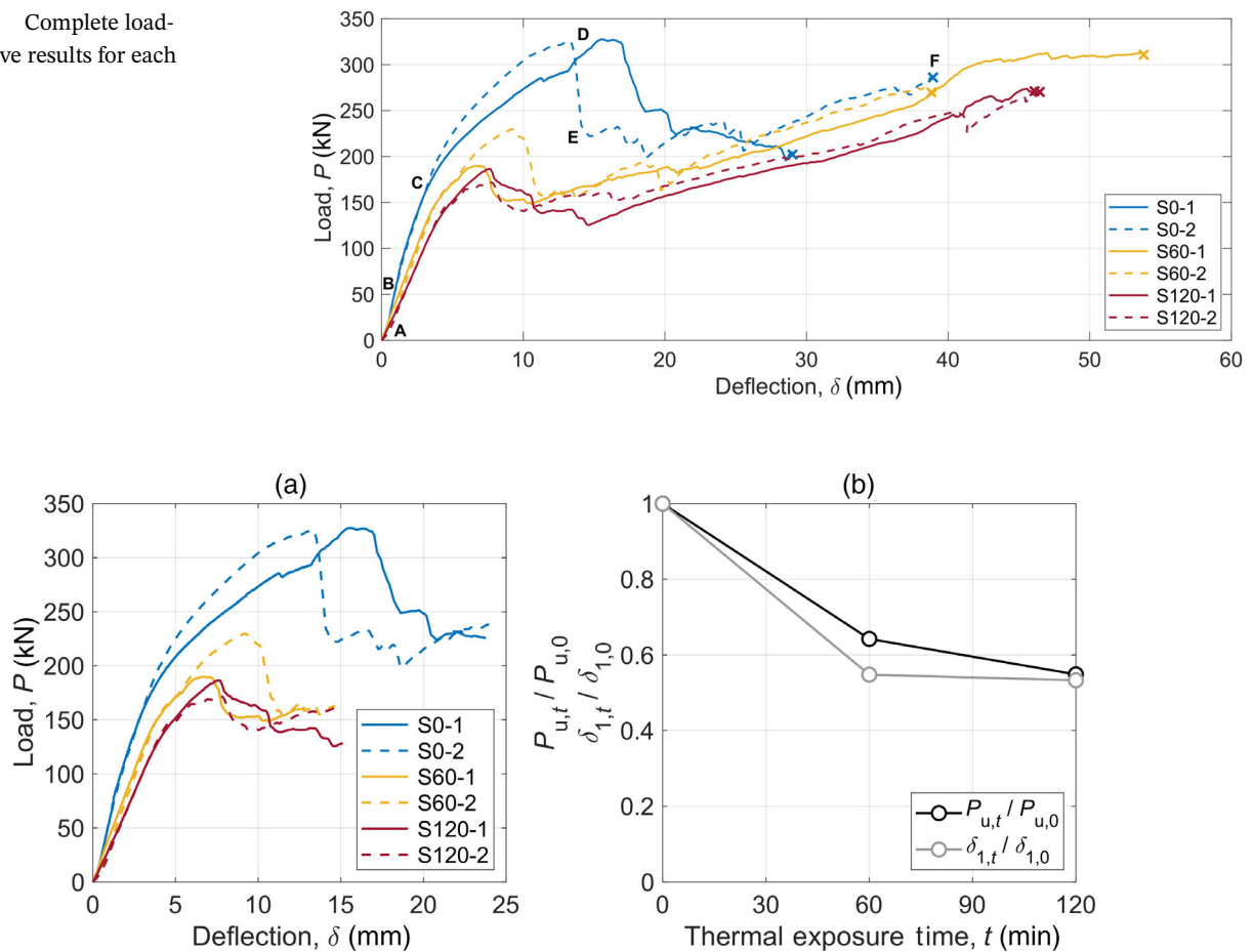
FIGURE 9 (a) Close-up of load-deflection curves and (b) comparison of average failure load and deflection at failure load for each exposure time
