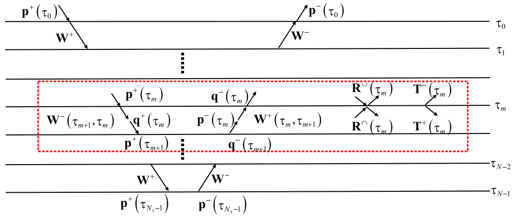
FIGURE 5 A schematic illustration of FWMod in pseudo-time. For the m th building block highlighted with a red square, \mathbf{p}^{\pm} are the incoming down-/up-going wavefields and \mathbf{q}^{\pm} are the outgoing down-/up-going wavefields; \mathbf{R}^{\cap/\cup} and \mathbf{T}^{\pm} denote downwards/upwards reflectivity and down-/up-going transmission operators, respectively; \mathbf{W}(\tau_{m+1}, \tau_m) and \mathbf{W}(\tau_m, \tau_{m+1}) represent the down-/up-going propagation operators.
