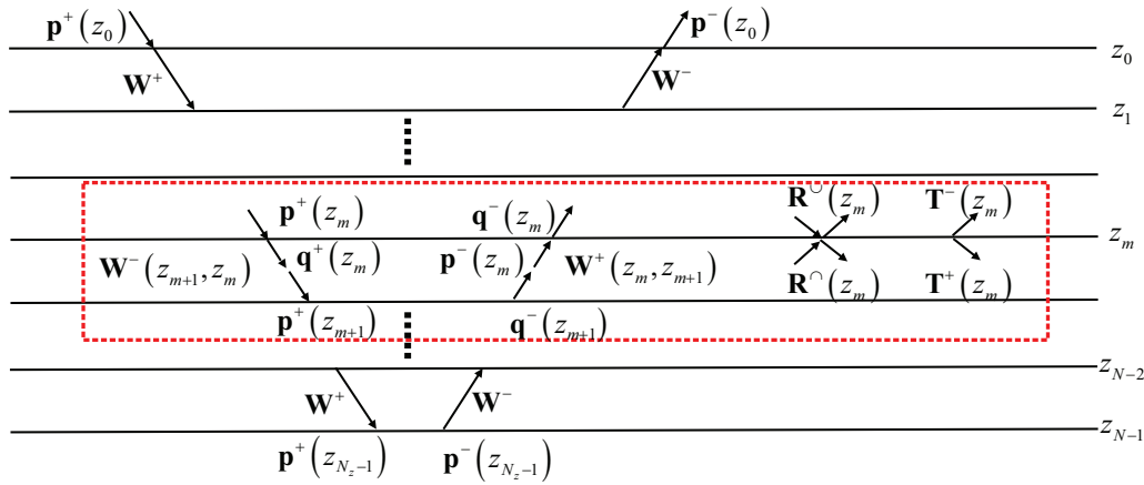
FIGURE 2 A schematic illustration of FWMod in depth. For the m th building block highlighted with a red square, \mathbf{p}^\pm are the incoming down-/up-going wavefields and \mathbf{q}^\pm are the outgoing down-/up-going wavefields; \mathbf{R}^{\cap/\cup} and \mathbf{T}^\pm denote downwards/upwards reflectivity and down-/up-going transmission operators, respectively; \mathbf{W}(z_{m+1}, z_m) and \mathbf{W}(z_m, z_{m+1}) represent the down-/up-going propagation operators.
