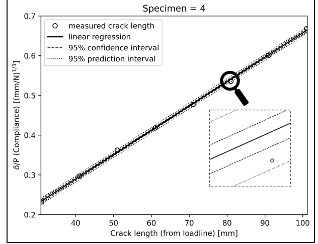
Figure 5. Compliance calibration.
