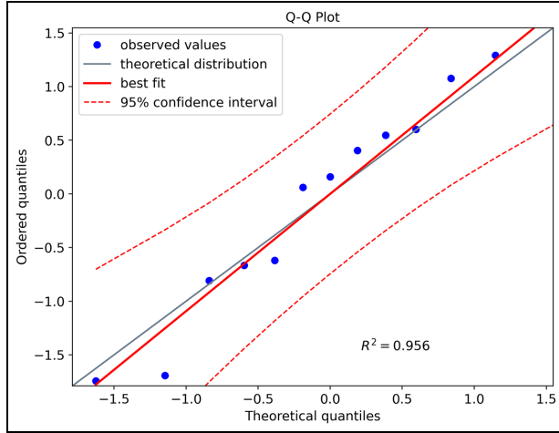
Figure 11. Darling-Anderson test.
