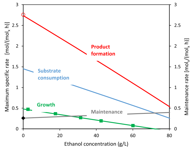
Fig. 2. Dependence of maximum specific rates (for growth, substrate consumption and product formation) and of maintenance rate, calculated for glucose fermentation to ethanol. Lines are calculations using kinetic parameters from Table 5 in Eqs. (1,9,10,13,14,16). Markers are literature data for growth and product formation [24] and for maintenance [91].
