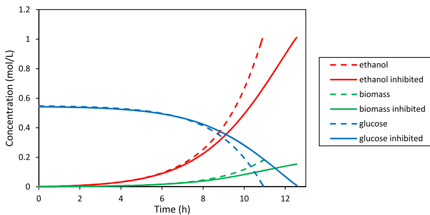
Fig. 3. Calculated batch reaction progress for glucose fermentation to ethanol, using the model given in the text, the parameters of Table 5, c_{s,feed} = 0.542 mol/L, and c_{x,feed} = 1 mmol/L. Dashed lines indicate the situation if product inhibition would not occur.
