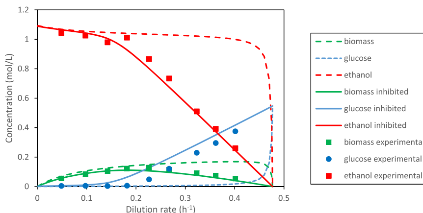
Fig. 4. Chemostat concentrations for glucose fermentation to ethanol for c_{s,feed} = 0.542 mol/L. Markers are experimental data [91]. Full lines are simulations using the model given in the text with the parameters of Table 5. Dashed lines indicate the simulated situation if product inhibition would not occur.
