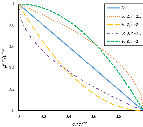
Fig. 1. Dependence of maximum specific growth rate on product concentration according to Eqs. (1–3).
