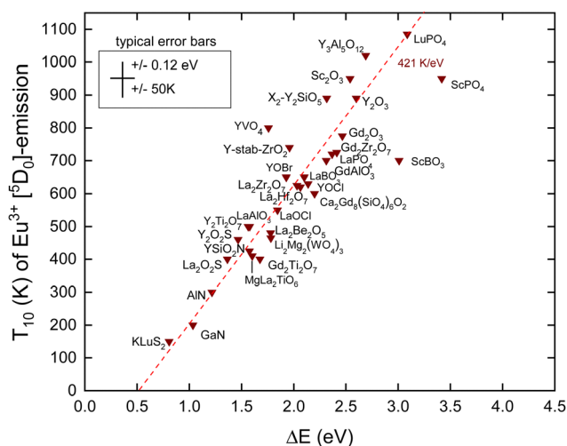
Fig. 4 10% Quenching temperature T_{10} for the \text{Eu}^{3+} emission from the {}^5\text{D}_0 level against the energy difference between the {}^5\text{D}_0 hole state and the VB-top. The fitted dashed line has a slope of 421 \text{ K eV}^{-1} .
