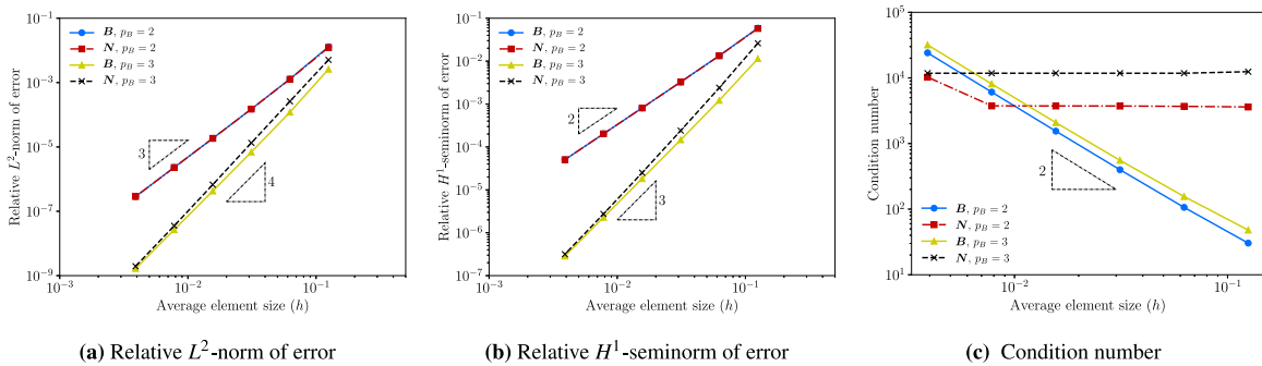
Fig. 15. One-dimensional Poisson–Dirichlet problem. Finite element convergence and condition number of the stiffness matrices for the C^1 continuous SB-splines N(\mathbf{x}) and the mixed smoothness B-splines B(\mathbf{x}) , consisting of C^0 and C^{p_B-1} continuous basis functions.
