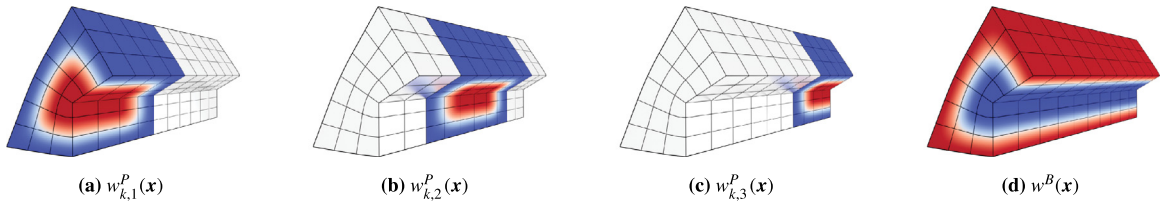
Fig. 12. Weight functions for the extraordinary prism. The weight functions w_{k,1}^P(x) , w_{k,2}^P(x) and w_{k,3}^P(x) are obtained by choosing three univariate weight functions w_{k,1}^{II}(\xi_3) , w_{k,2}^{II}(\xi_3) and w_{k,3}^{II}(\xi_3) along the centre of the extraordinary prism as depicted in Fig. 11(b). The weight function w^B(x) is their complement to one, i.e. w^B(x) = 1 - w_{k,1}^P(x) - w_{k,2}^P(x) - w_{k,3}^P(x) . The scalar field ranges between 0 (blue) and 1 (red). (For interpretation of the references to colour in this figure legend, the reader is referred to the web version of this article.)
