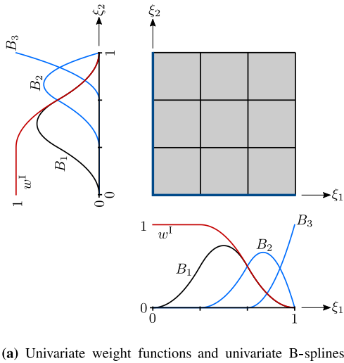
Fig. 8. Construction of the weight function w^Q(x) on one of the v sectors in the 3-neighbourhood of an extraordinary vertex. The weight function w^Q(\xi) on the parametric domain \hat{\Omega} is defined as the product of the univariate weight functions w^1(\xi_1) and w^1(\xi_2) in (a). Formally, w^Q(x) on each element on the domain \Omega in (b) is given by w^Q(x) = w^Q(\xi) \circ \eta(\xi)^{-1} \circ x(\eta)^{-1} .
