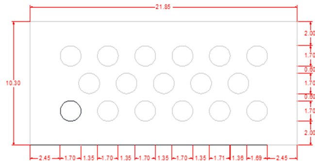
Fig. 5. S/BP brick dimensions.
