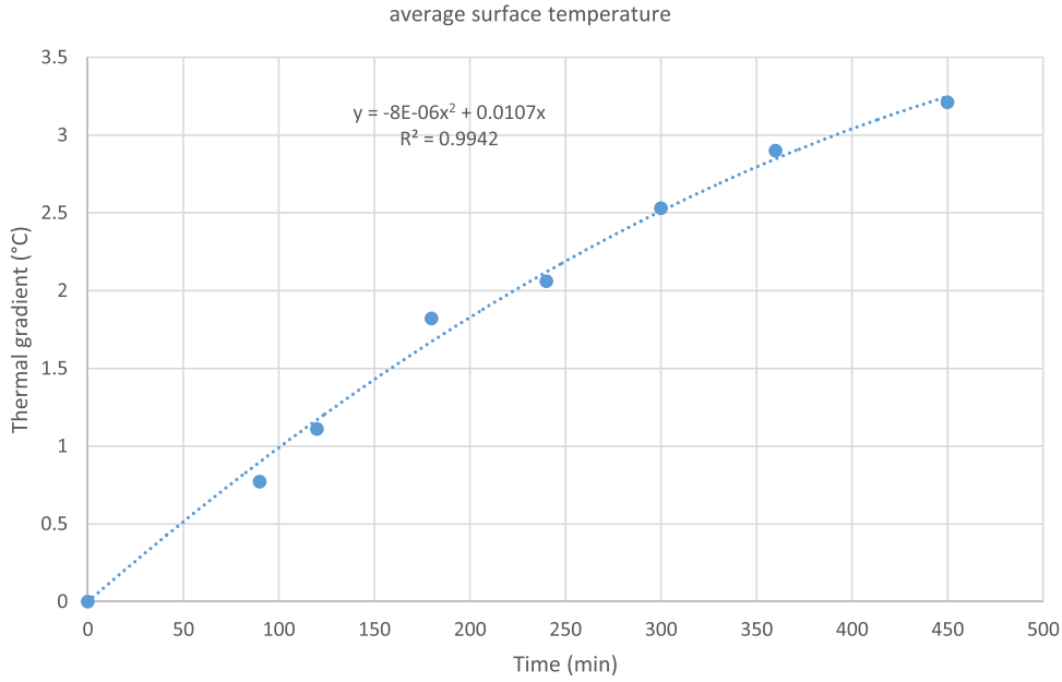
Fig. 17. Average surface temperature variation of side wall exposed to ambient temperature.
