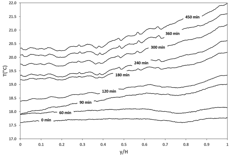
Fig. 18. Wall surface temperature gradients with respect to height and time.
