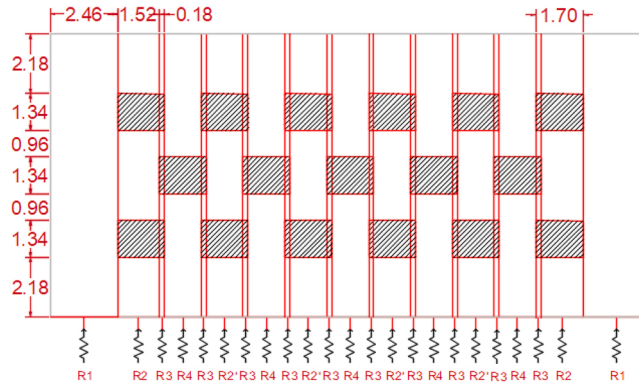
Fig. 9. Equivalent simplified scheme of S/BP brick.
