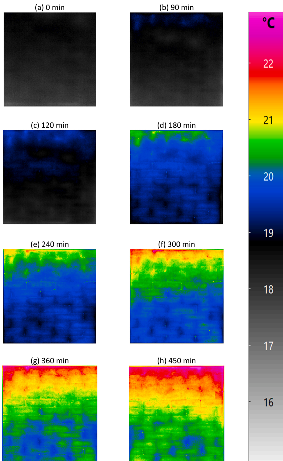
Fig. 19. Visible images by thermography that depict the distribution of temperature differences on the S/BP wall surface exposed to ambient temperature and recorded at: (a) 0 min, (b) 90 min, (c) 120 min, (d) 180 min, (e) 240 min, (f) 300 min, (g) 360 min, (h) 450 min.
