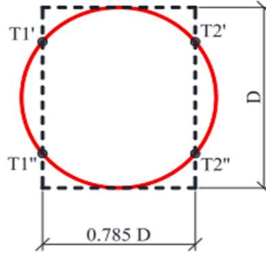
Fig. 6. Determination of the equivalent thickness of a cylindrical cavity.
