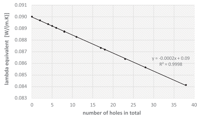
Fig. 4. Impact of holes number in a S/BP brick on the equivalent thermal conductivity.
