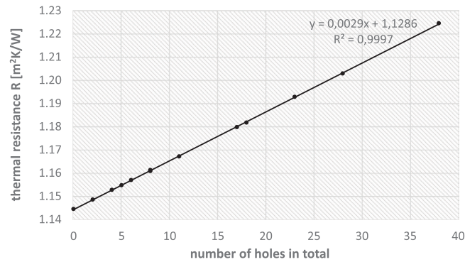
Fig. 3. Impact of holes number in a S/BP brick on the equivalent thermal resistance.
