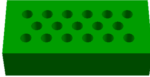
Fig. 2. Hollow brick design for i = 3 and j = 6 .
