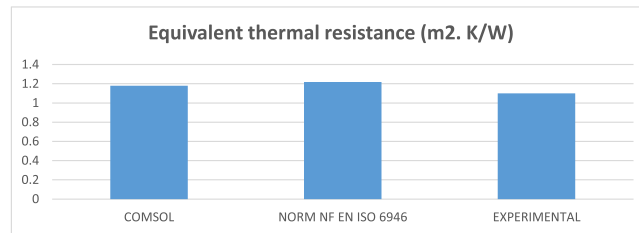
Fig. 14. Equivalent thermal resistance comparison between numerical and experimental of S/BP composite.
