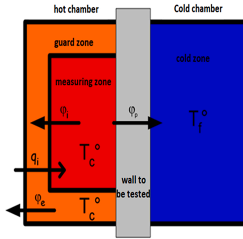
Fig. 13. heat transfer inside a bi-climatic chamber.
