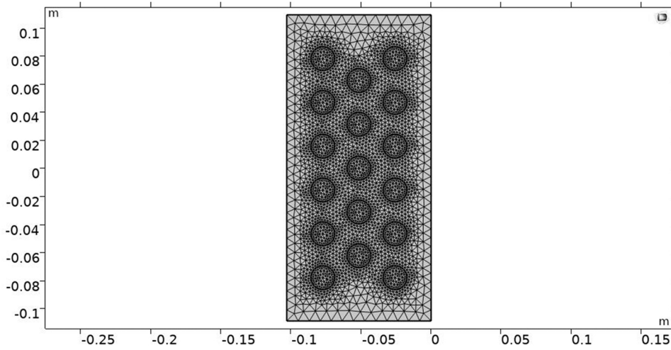
Fig. 1. Physics-controlled mesh for “finer” mesh size in COMSOL of the design for i = 3 and j = 6 .
