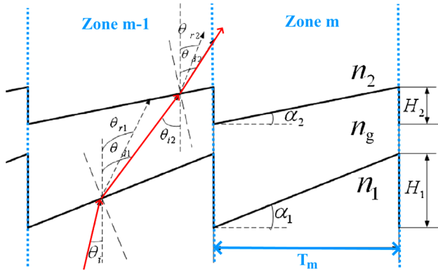
Fig. 1. Extended scalar theory applied to an MLDOE (adapted from [11]). The deviation angle \theta_d is obtained using the local grating equation, while \theta_r results from Snell's law. Initially, the layer heights H_1 and H_2 are constant, given by the TEA. EST alternative profile heights are obtained when \theta_d = \theta_r for both layers. T_m is the m th zone period. The light trajectory is displayed in red.
