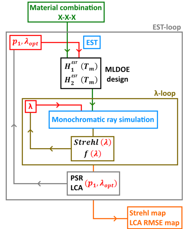
Fig. 4. Diagram describing the proposed MLDOE thickness optimization algorithm. It is divided into two loops and searches the “best” EST input doublet (p_1, \lambda_{opt}) . A set of layer materials and a pair (p_1, \lambda_{opt}) defines an “MLDOE design.” The green loop involves the ray model and Fig. 2 diagram. It is performed over the MWIR-LWIR wave bands. At the end of the loop, the polychromatic Strehl ratio (PSR) is obtained for each pair (p_1, \lambda_{opt}) . This process is repeated in the main loop (gray) for each value of (p_1, \lambda_{opt}) , resulting in either a PSR curve [if Eq. (4) is applied] or a PSR two-dimensional map. This output map (or curve) is specific for each MLDOE material combination, given the above-mentioned global parameters.
