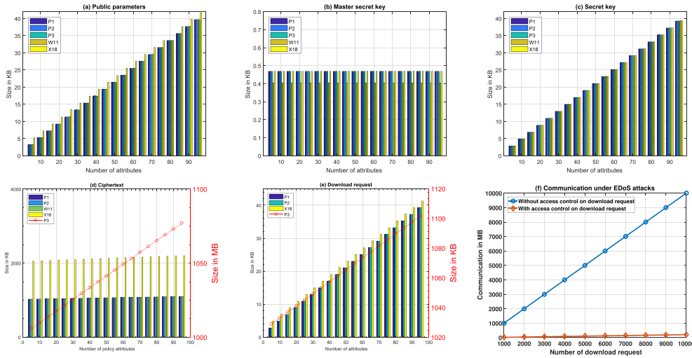
Fig. 3. Experimental results in terms of communication cost.
