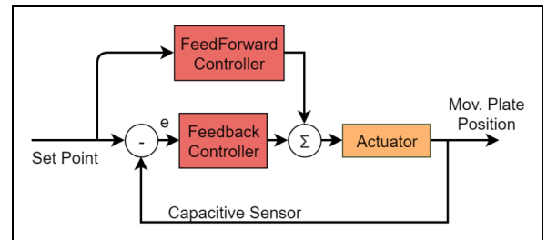
Figure 14. Movable plate control strategy (ILC).
